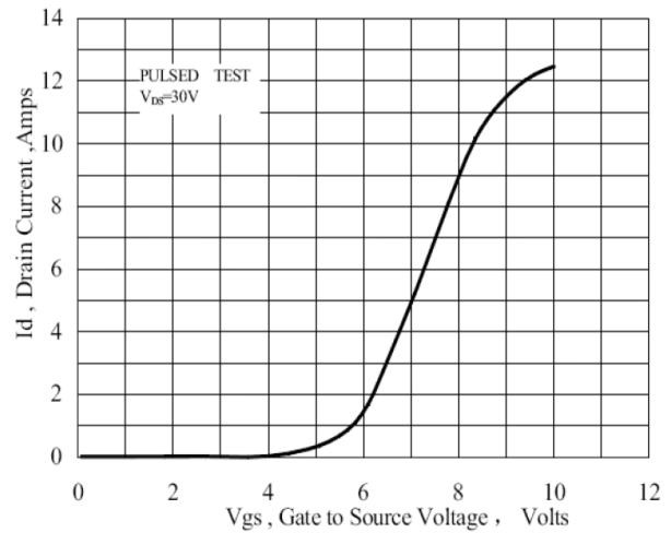
Fig 8 Transfer Characteristics
