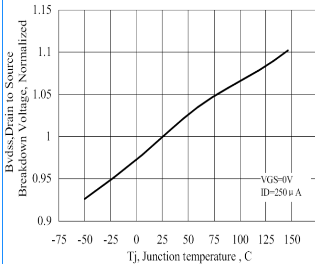
Fig 11 Normalized Breakdown Voltage vs. Junction Temperature
