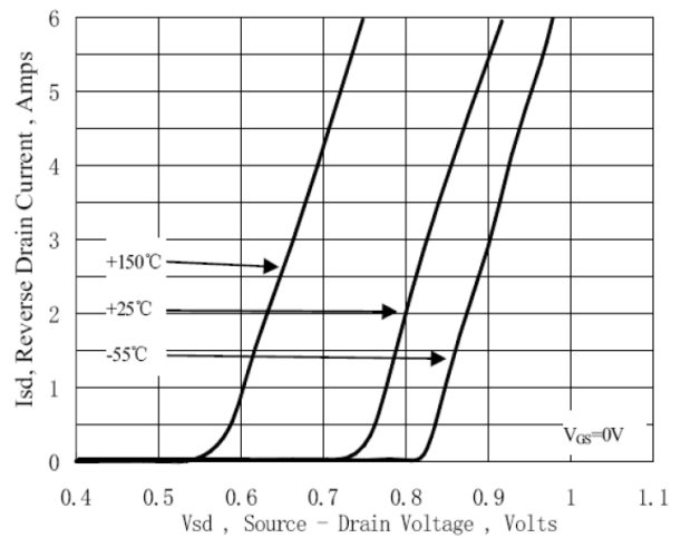
Fig 6 Body-Diode Characteristics
