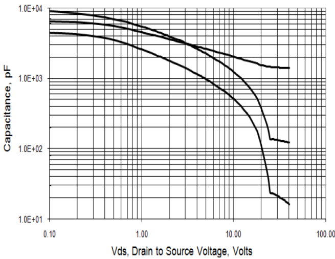
Fig 9 Capacitance Characteristics
