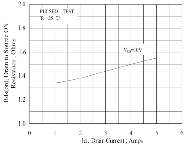
Fig 4 On-Resistance vs. Drain Current and Gate Voltage
