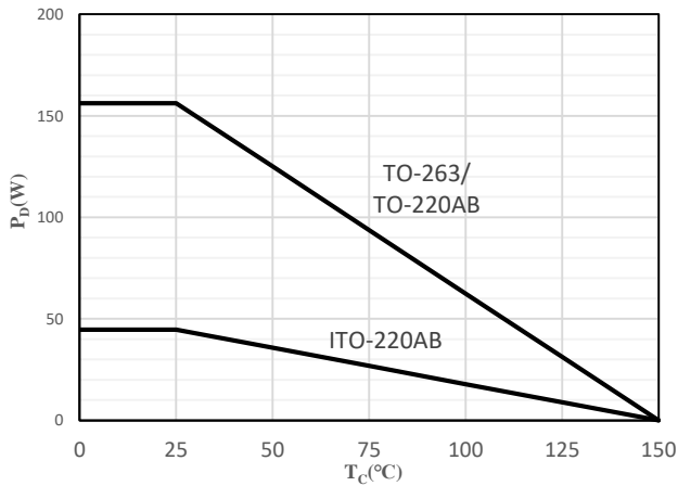
Fig 1 Power Dissipation
