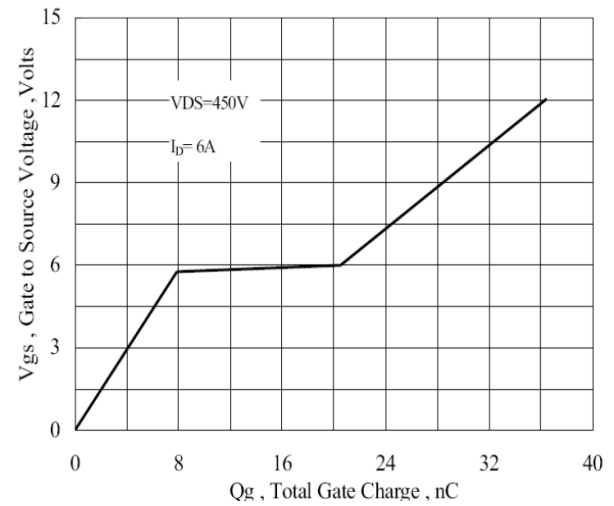
Fig 10 Gate-Charge Characteristics
